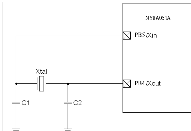
Figure 17 Connection for External Crystal Oscillation
