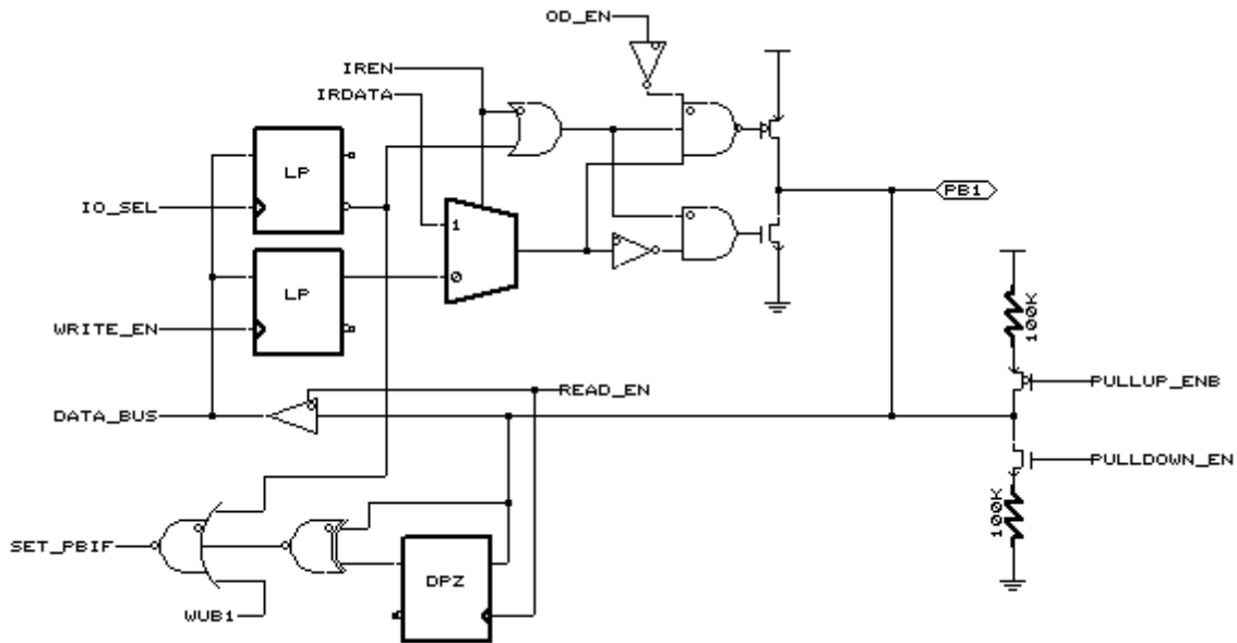
Figure 6 Block Diagram of PB1
