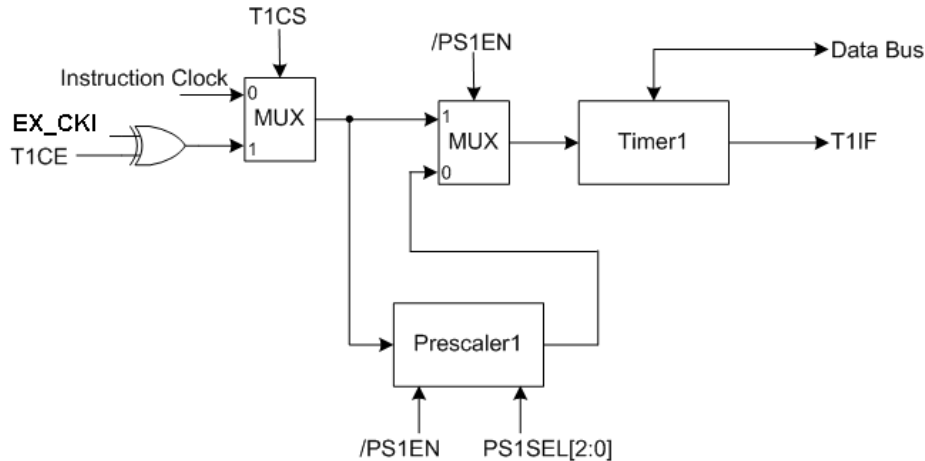
Figure 11 Block Diagram of Timer1
