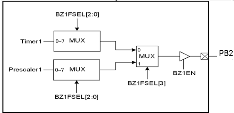
Figure 14 Buzzer1 Block Diagram
