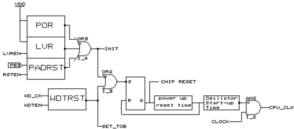
Figure 19 Block diagram of on-chip reset circuit
