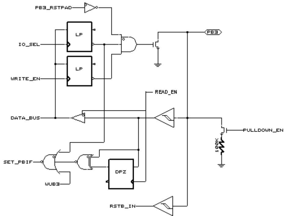
Figure 8 Block Diagram of PB3
