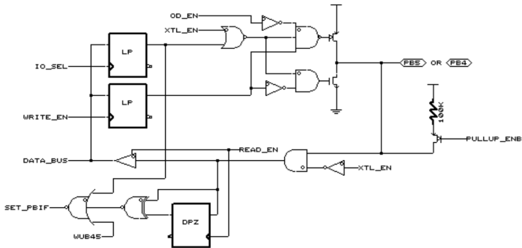
Figure 9 Block Diagram of PORT PB4/PB5
