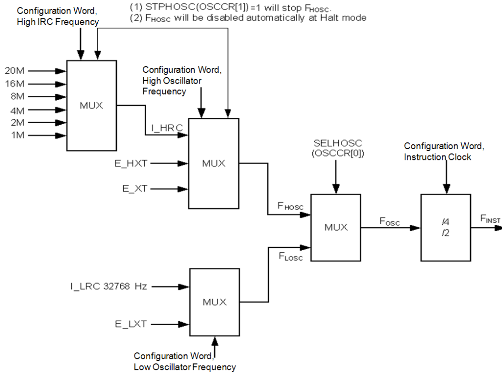
Figure 16 Oscillation Configuration of NY8A051A
