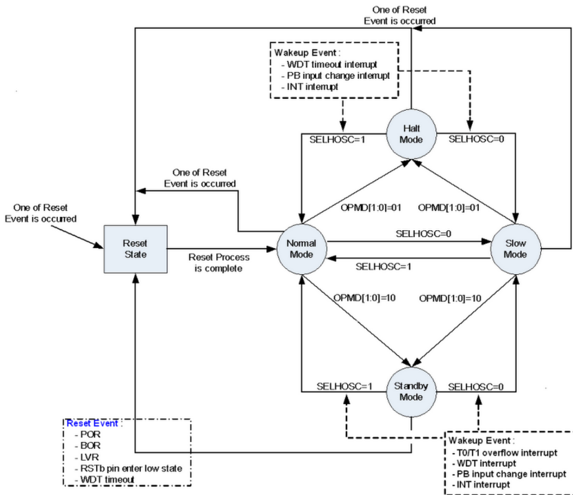
Figure 18 Four Operating Modes
