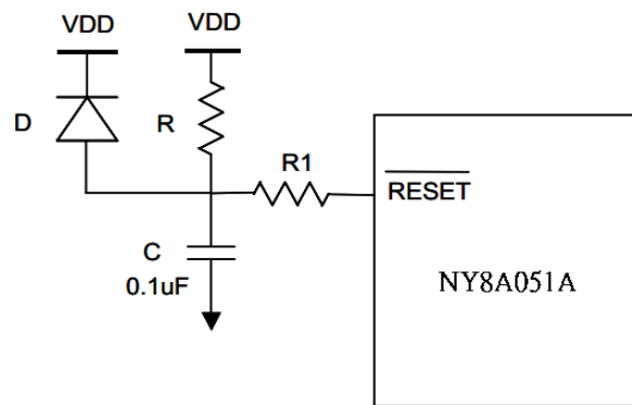
Figure 20 Block Diagram of reset application
