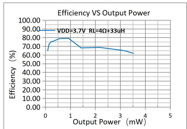
图 6. Efficiency VS Output Power
