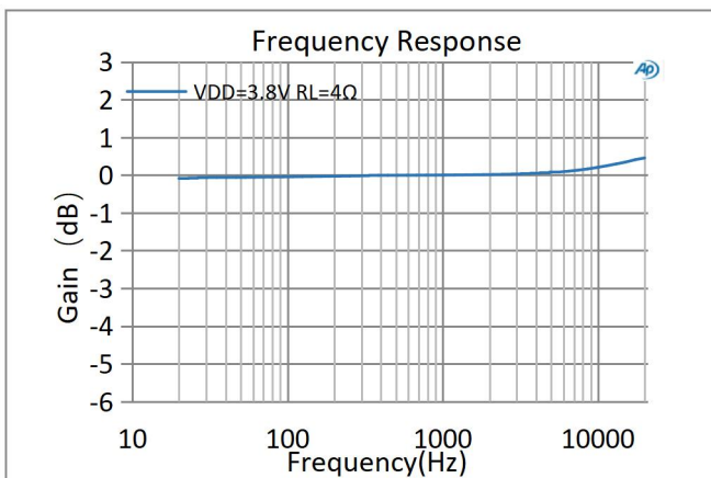
图 5. Frequency Response
