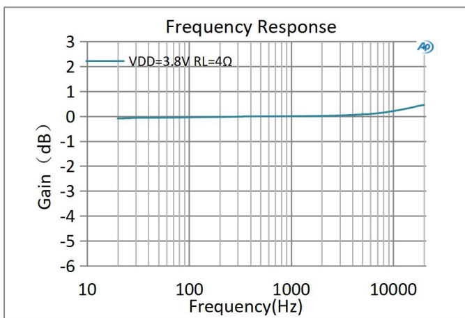
图5: Frequency Response
