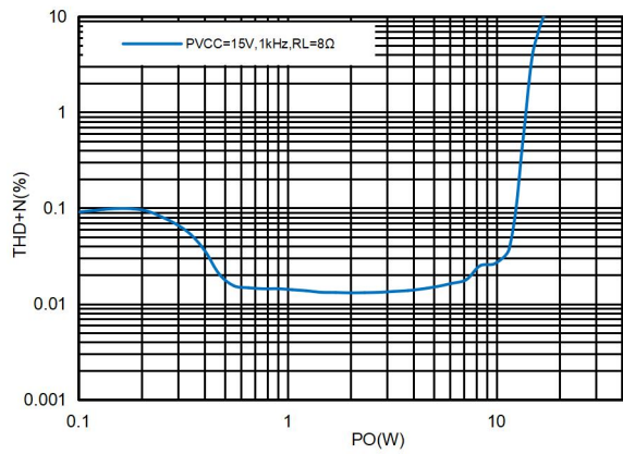
图34. 15V供电8Ω负载THD+N曲线PBTL
